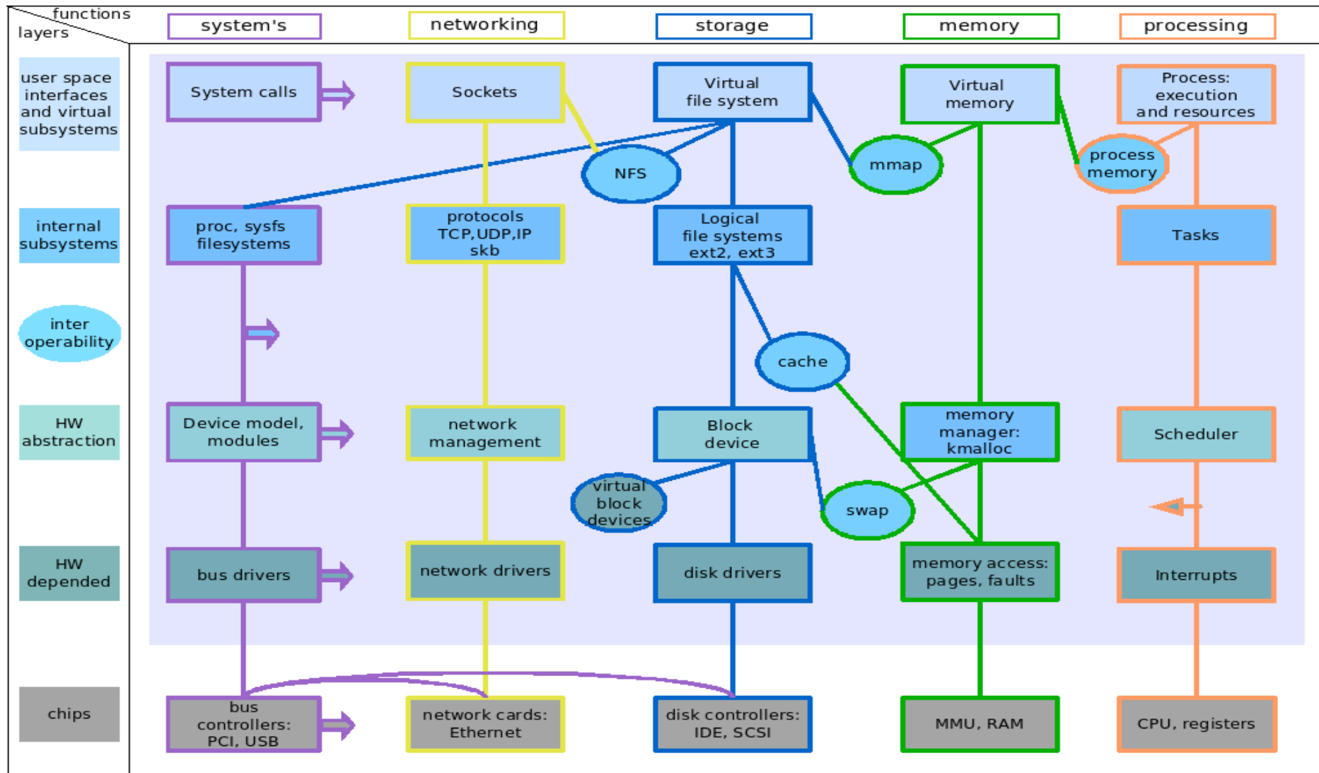
Simplified Linux kernel diagram in form of a matrix map
